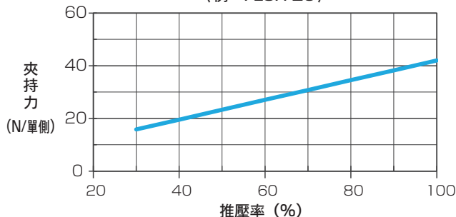
夾持力和推壓率 (例: FLSH-20)
