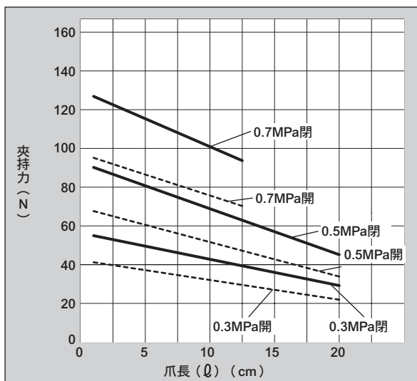
● CKJ-16CS
