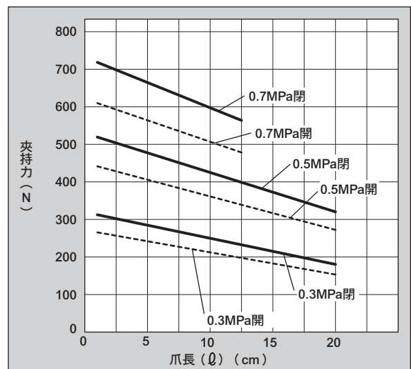
● CKJ-40CS
